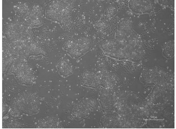
CiRA-jk-0118-D: passage-3
