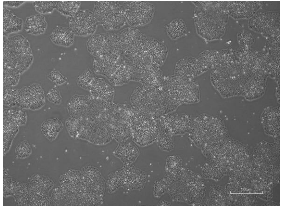
CiRA-jk-0118-F: passage-3
